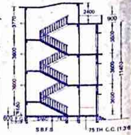
SECTION AT XX SCALE 1:75
